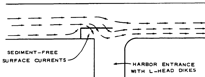
Figure 12-4. L-head dike used to reduce shoaling in harbor entrance
