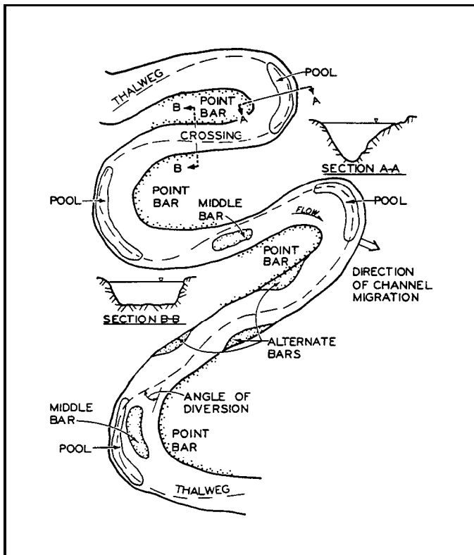
Figure 7-5. Channel planform
