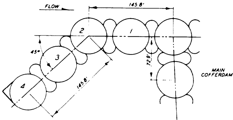
Figure 11-2. Cofferdam deflector
