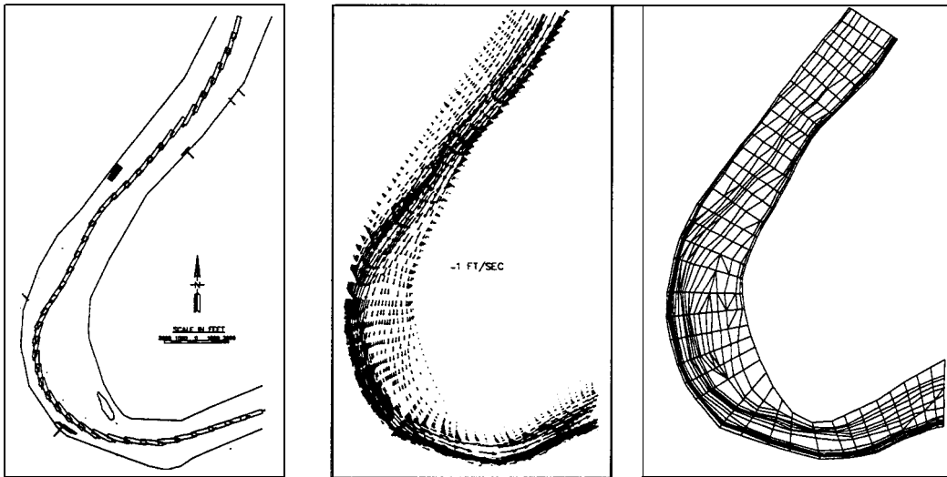
a. WES tow simulator track plots b. RMA2-WES hydrodynamic solution c. Numerical model computational mesh
